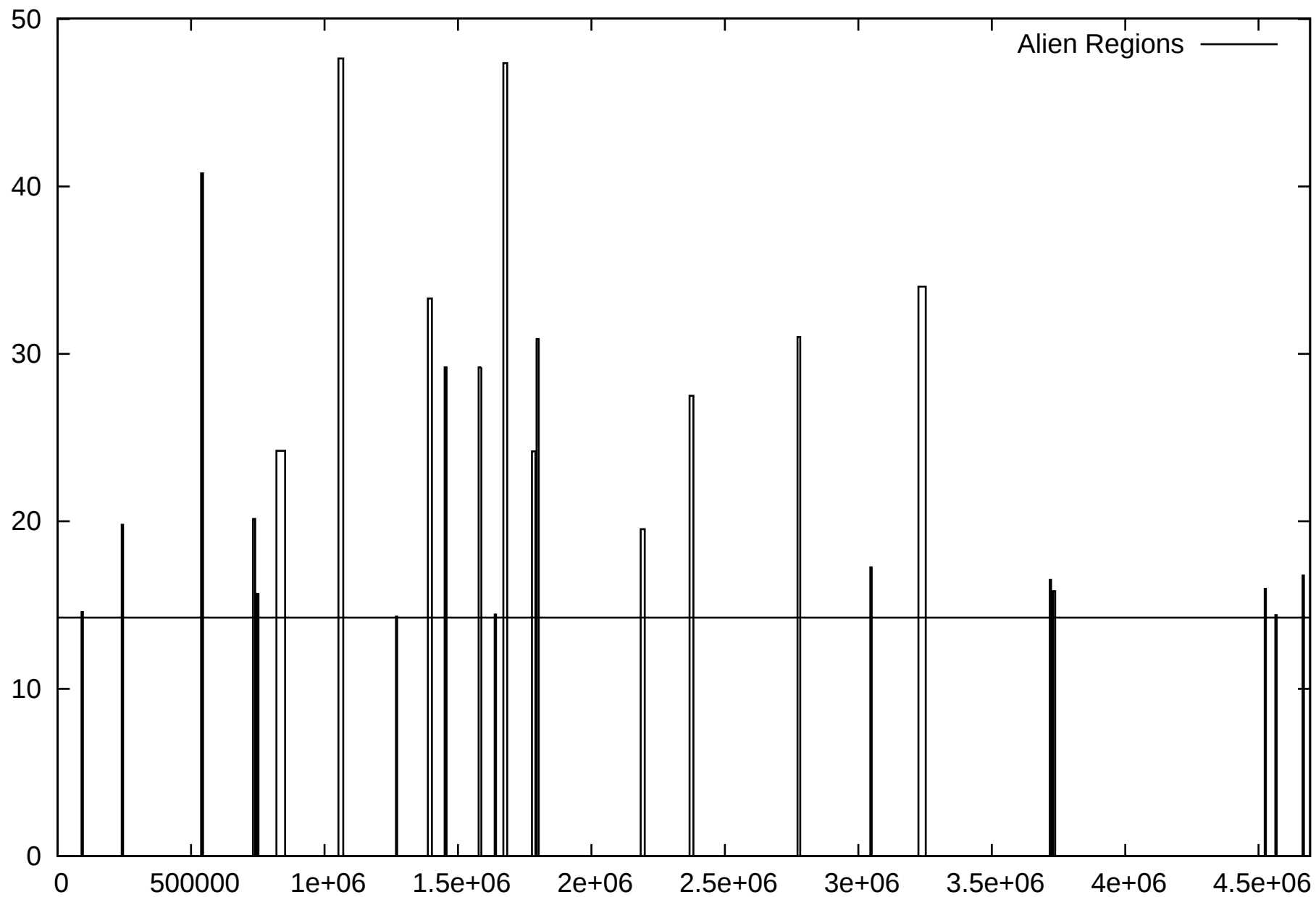
Xarb_fragariae_CFBP6773 Alien Regions
