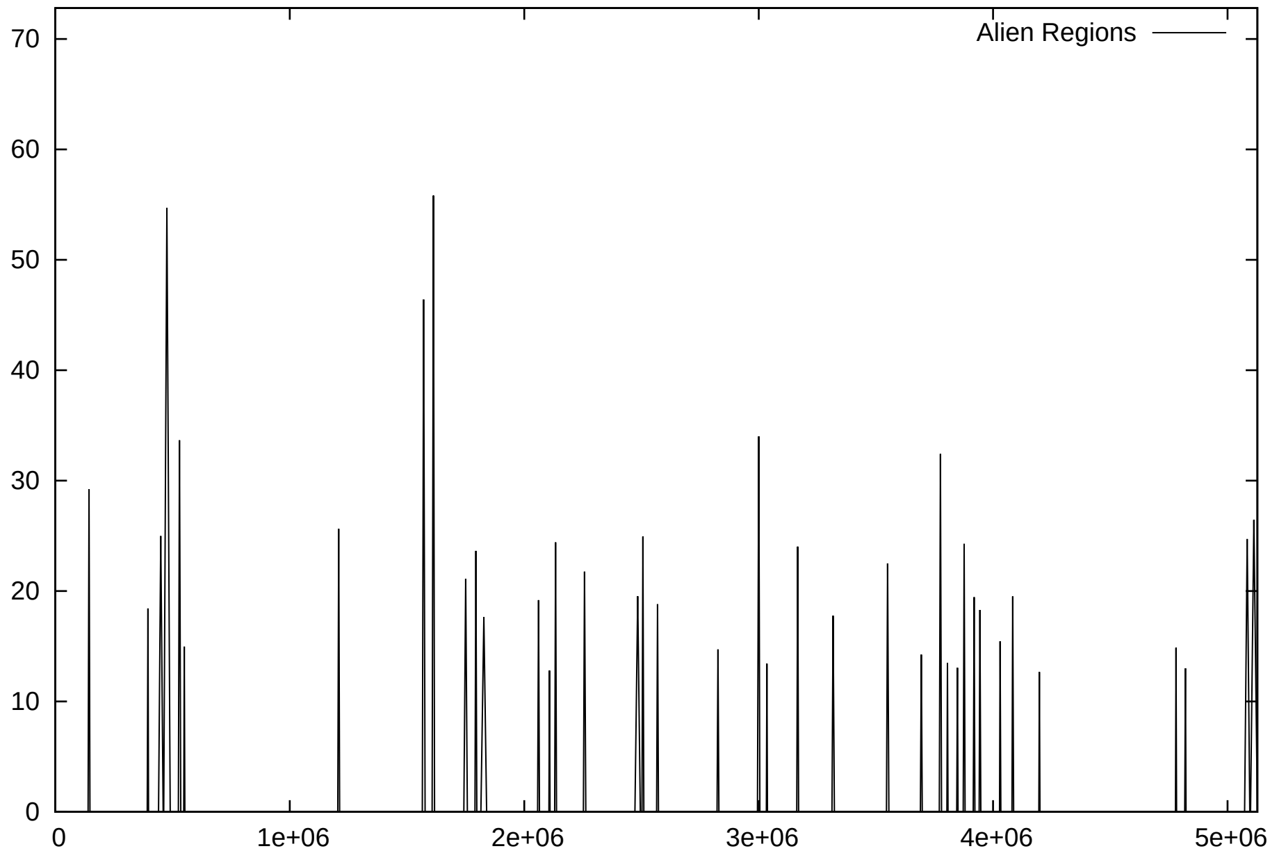
Alien Regions of S_marcences_RSC14
