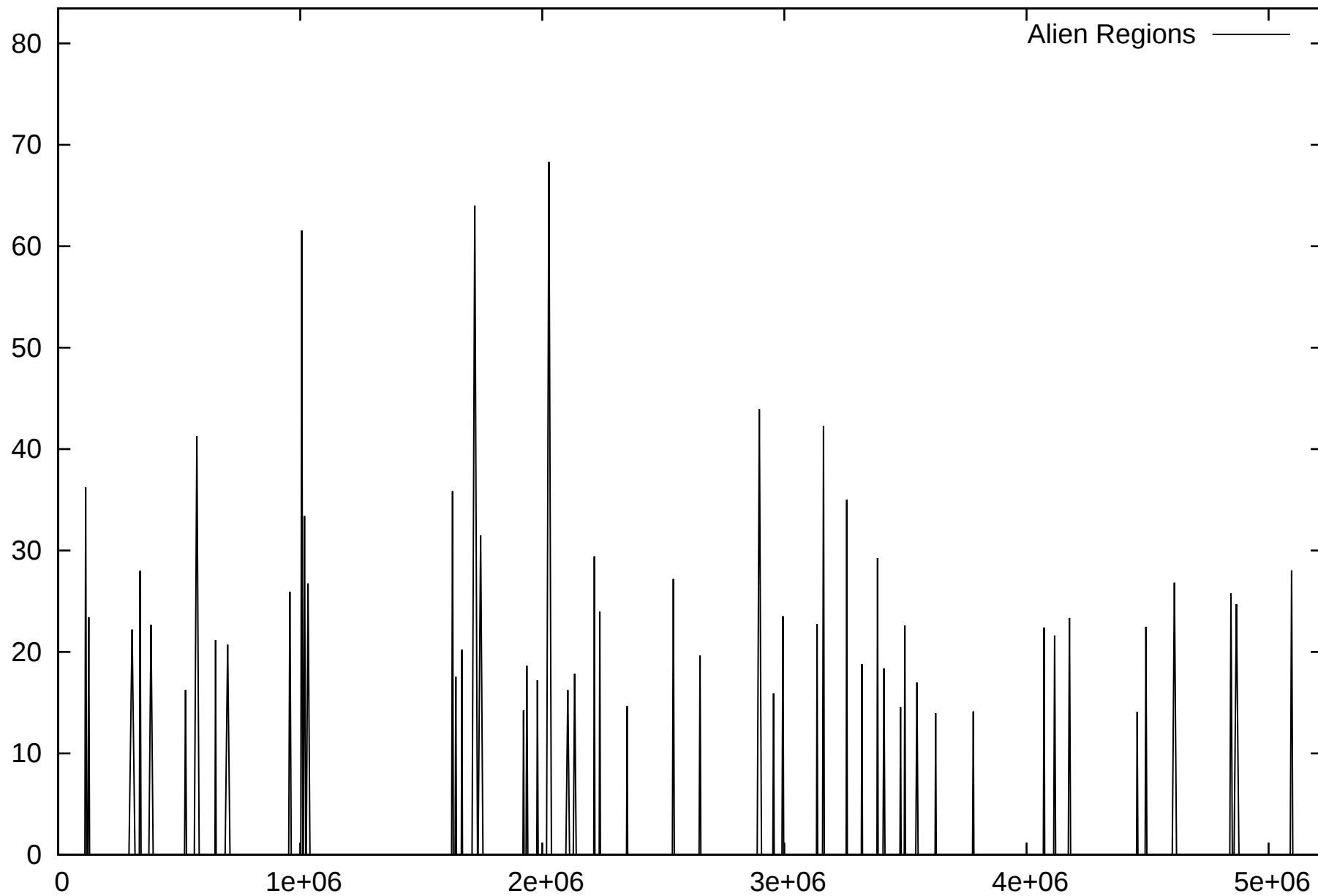
Alien Regions of S_marcences_WW4
