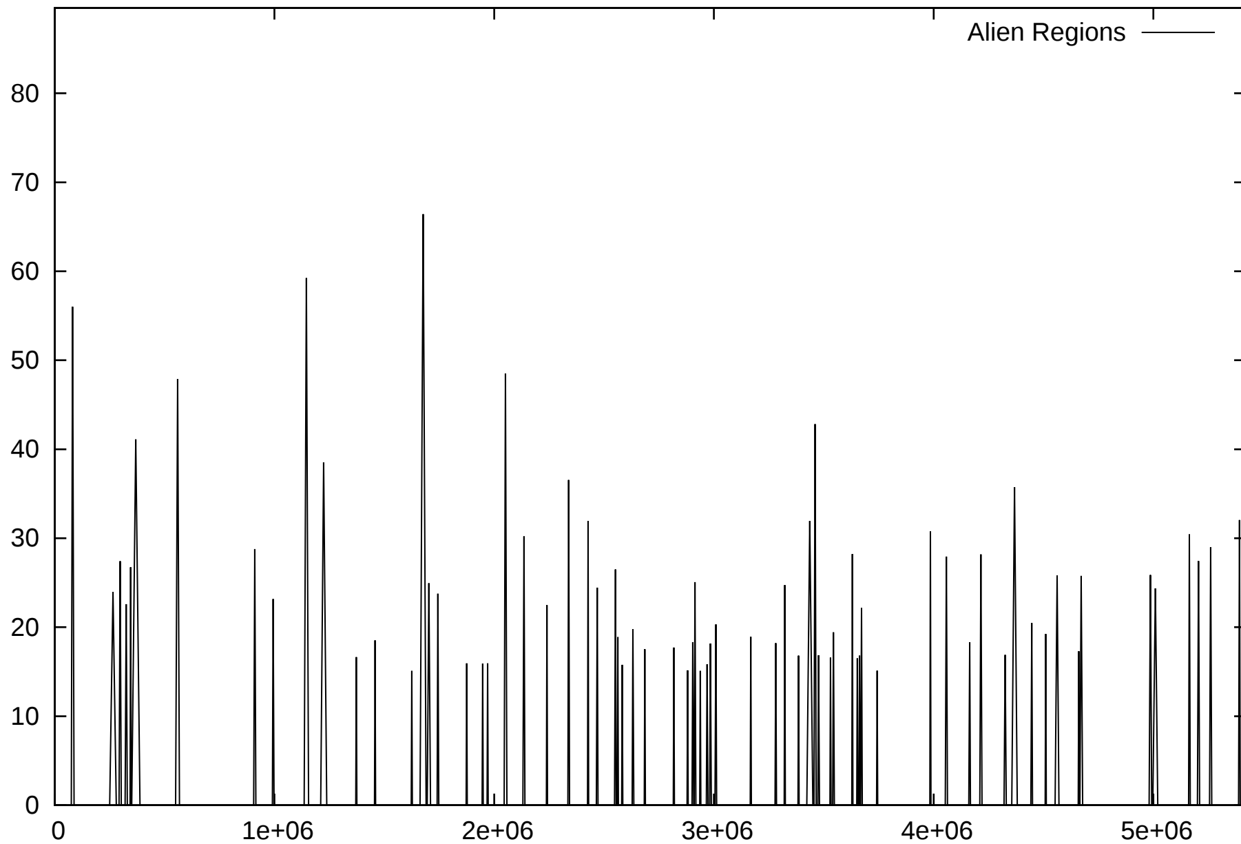
Alien Regions of S_sp_AS13
